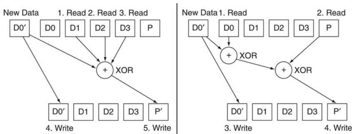
FIGURE E5.11.2 Small write update on RAID 4.
