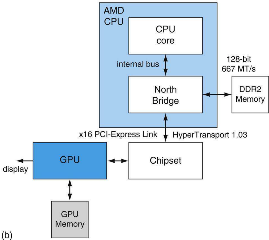
FIGURE B.2.2 Contemporary PCs with Intel and
