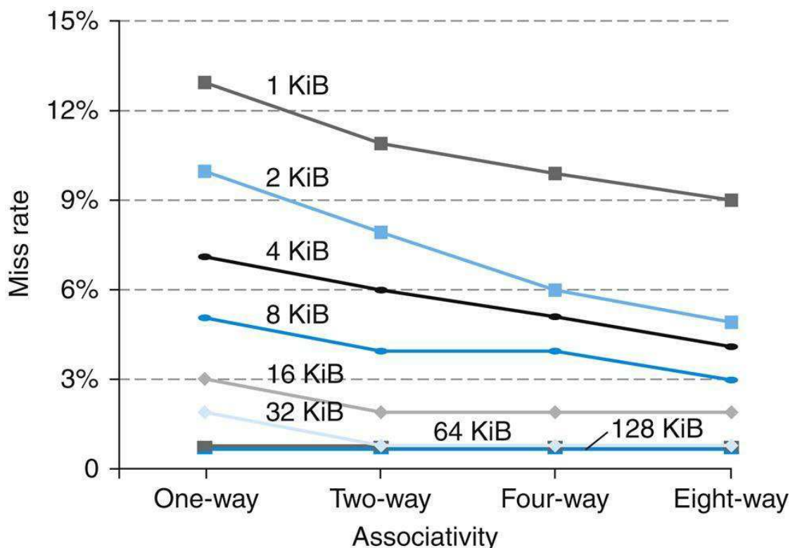
FIGURE 5.35 The data cache miss rates for each of eight cache sizes improve as the associativity increases.
