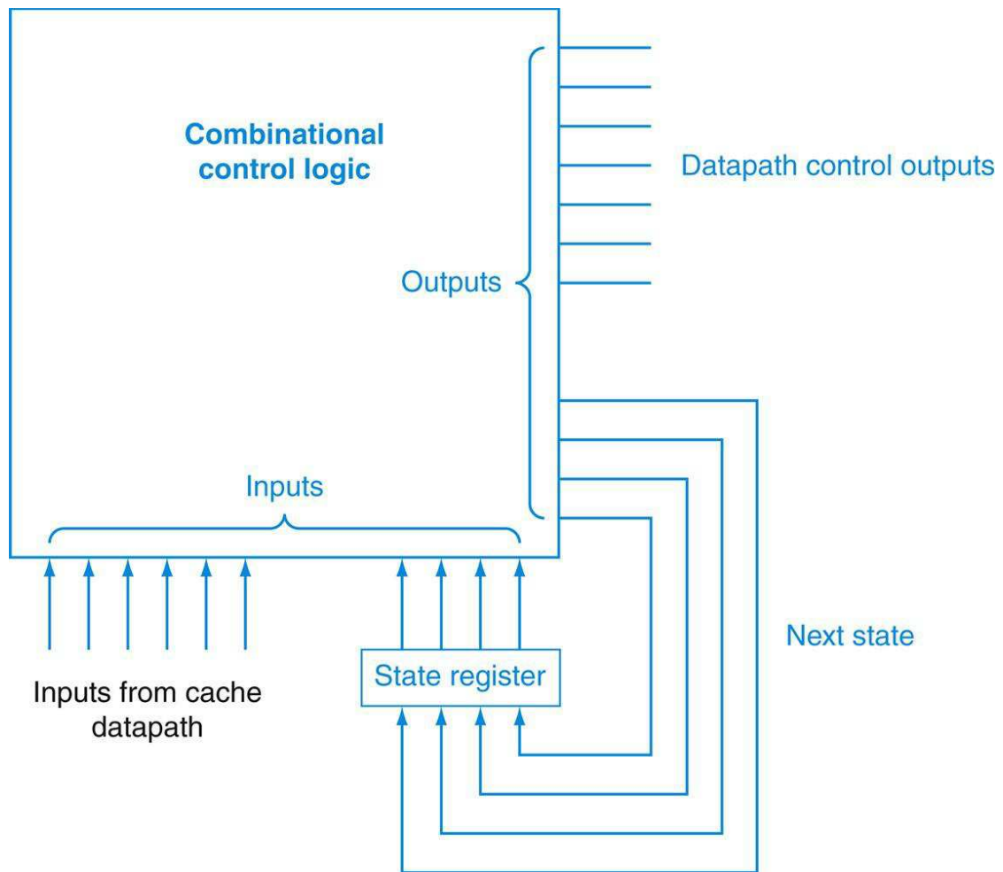
FIGURE 5.38 Finite-state machine controllers are typically implemented using a block of combinational logic and a register to hold the current state.
