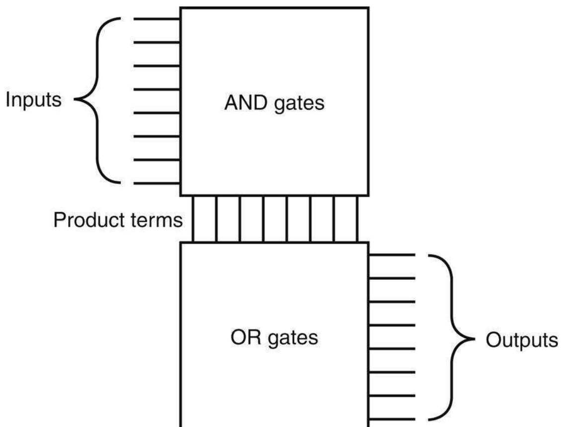
FIGURE A.3.3 The basic form of a PLA consists of an array of AND gates followed by an array of OR gates.
