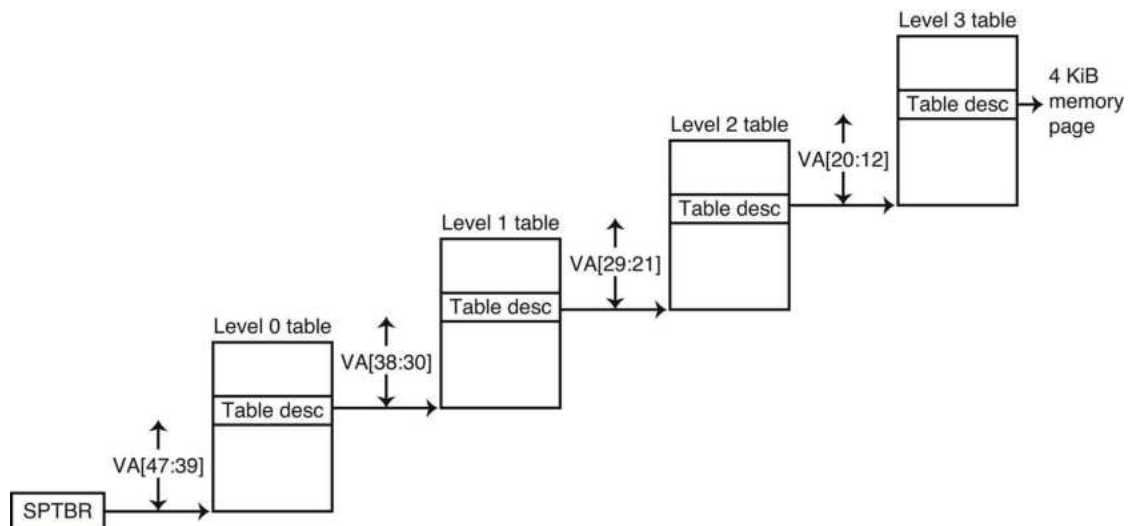
FIGURE 5.29 RISC-V uses four levels of tables to translate a 48-bit virtual address into a 40-bit physical address.
