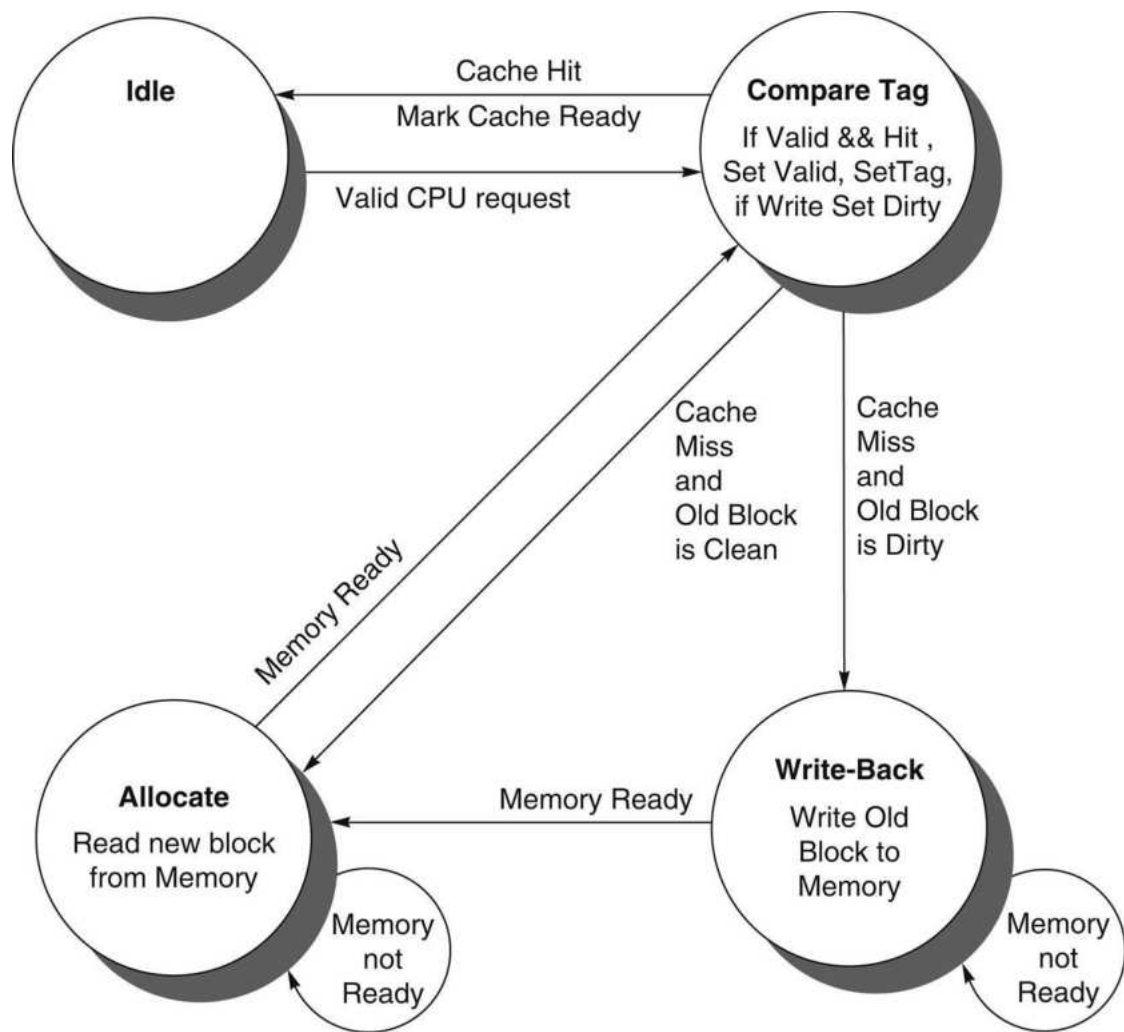
FIGURE 5.39 Four states of the simple controller.
