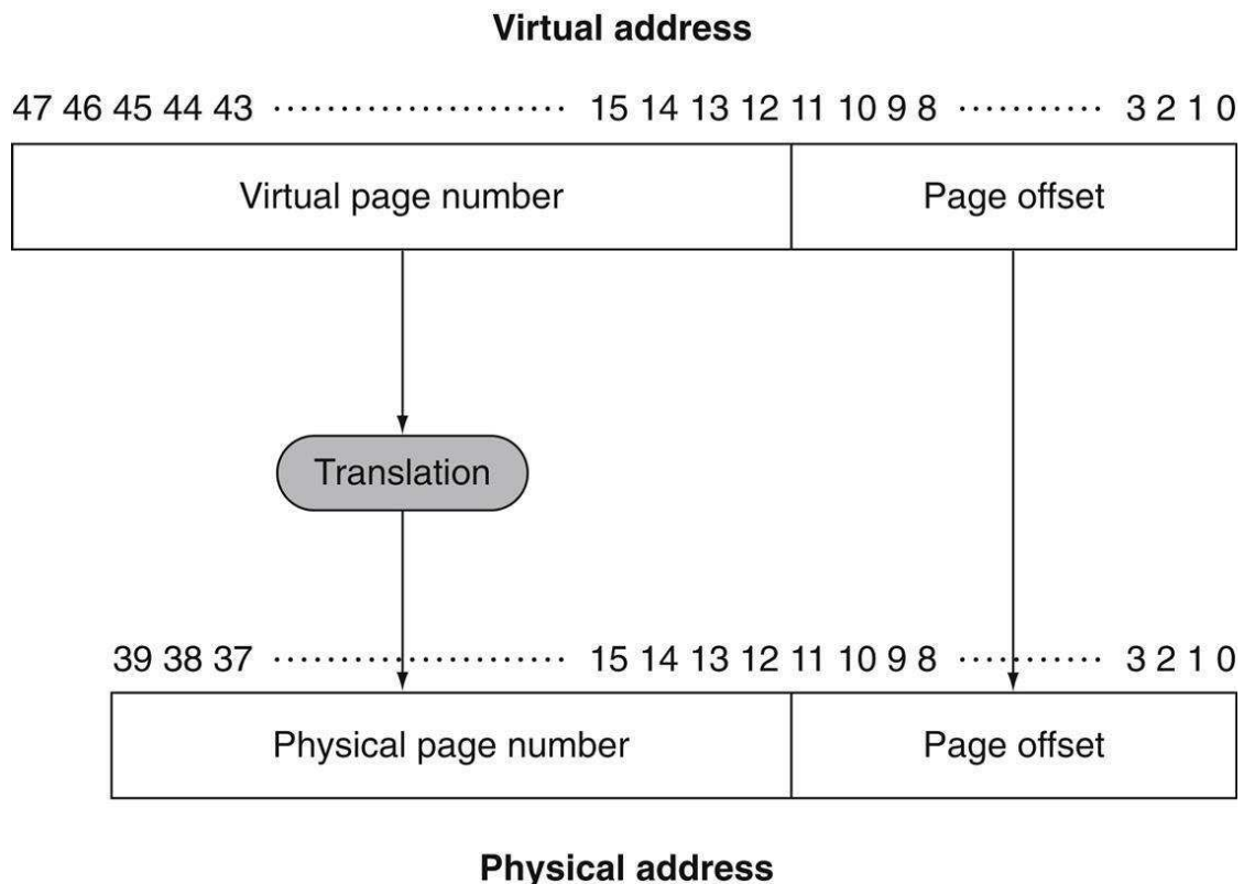
FIGURE 5.26 Mapping from a virtual to a physical address.
