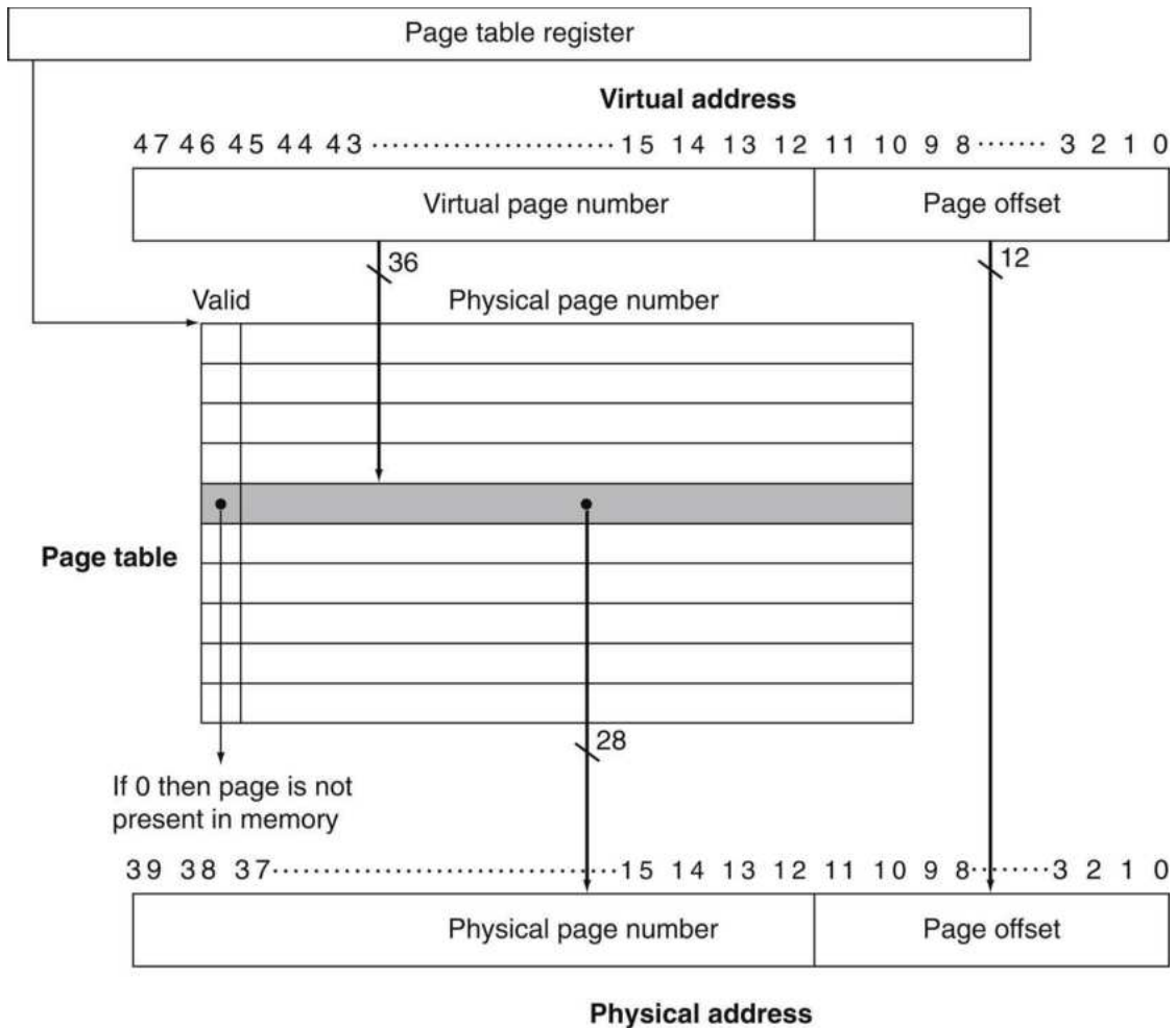
FIGURE 5.27 The page table is indexed with the virtual page number to obtain the corresponding portion of the physical address.
