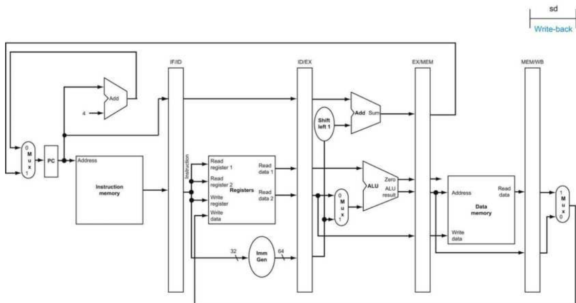
FIGURE 4.38 MEM and WB: The fourth and fifth pipe stages of a store instruction.
