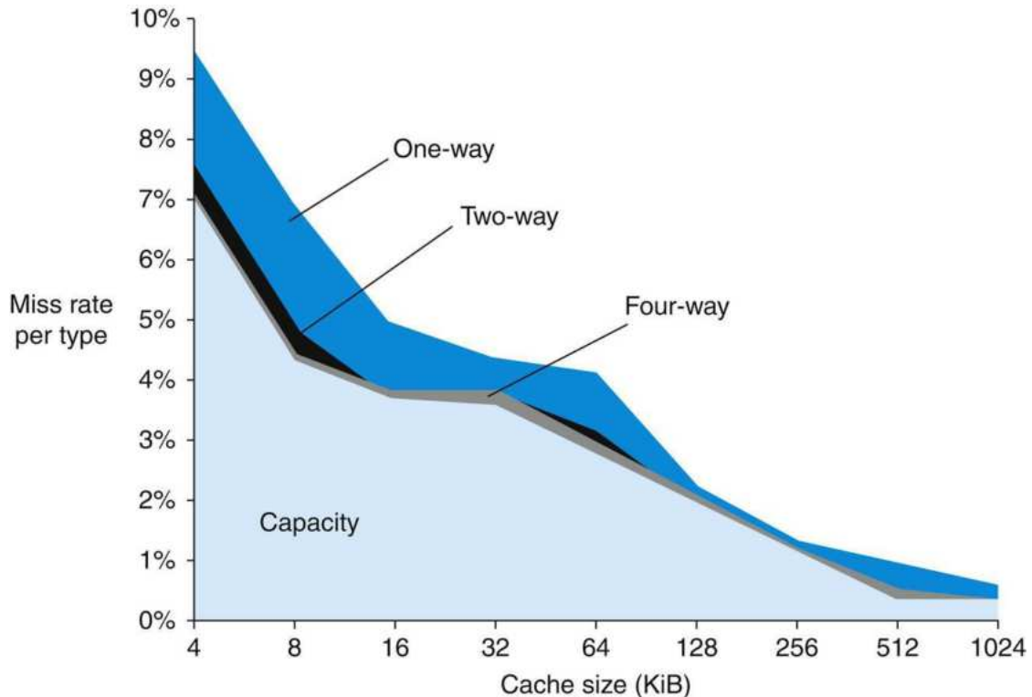
FIGURE 5.36 The miss rate can be broken into three sources of misses.
