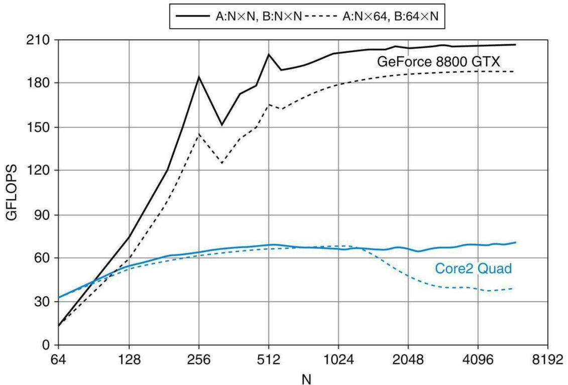
FIGURE B.7.3 SGEMM dense matrix-matrix multiplication performance rates.
