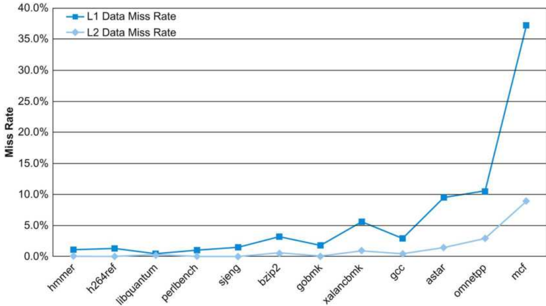
FIGURE 5.44 Data cache miss rates for ARM Cortex-A53 when running SPEC2006int.
