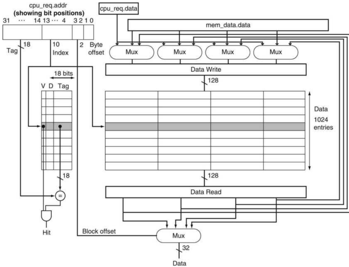
FIGURE E5.12.3 Block diagram of the simple cache using the Verilog names.
