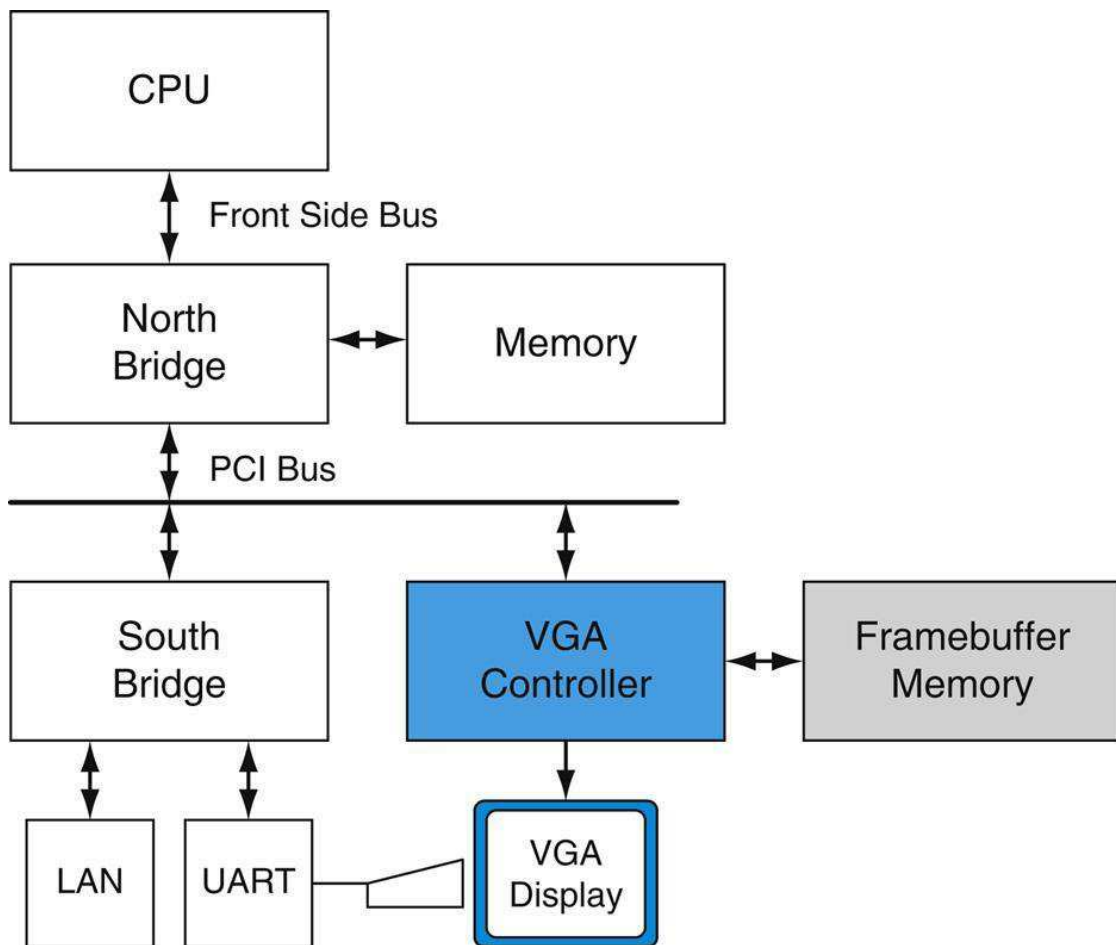
FIGURE B.2.1 Historical PC.
