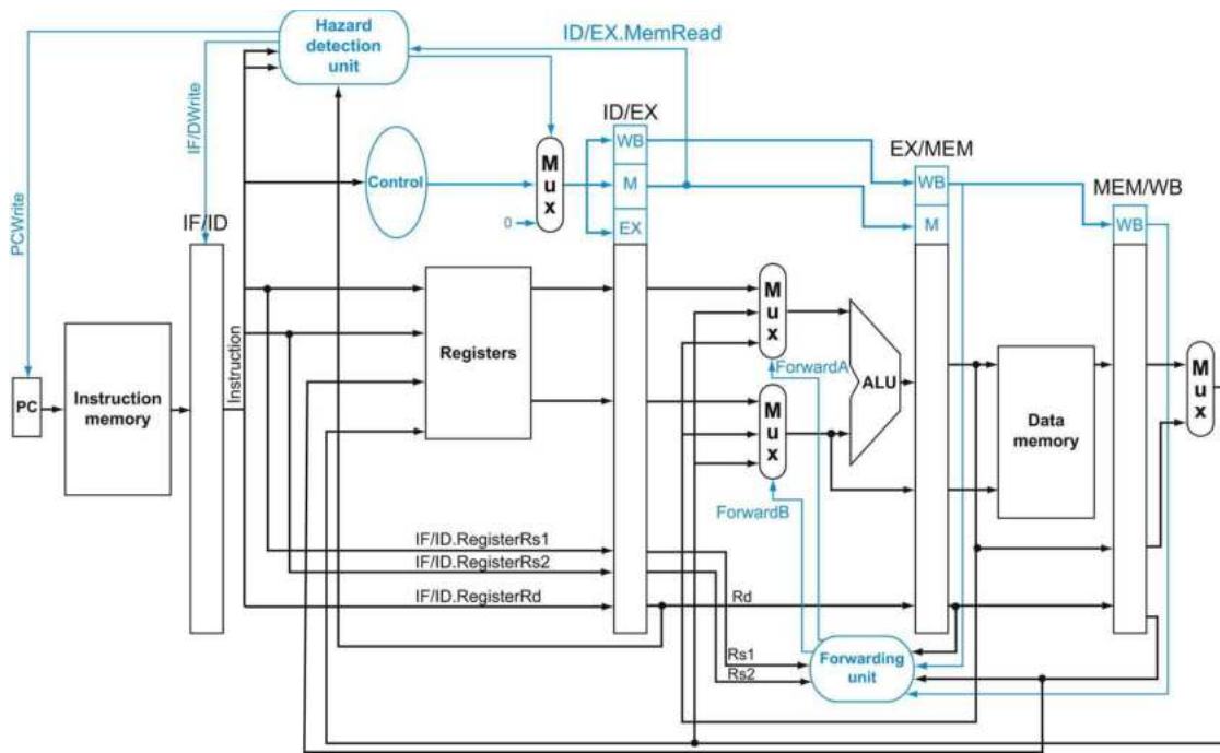
FIGURE 4.58 Pipelined control overview, showing the two multiplexers for forwarding, the hazard detection unit, and the forwarding unit.
