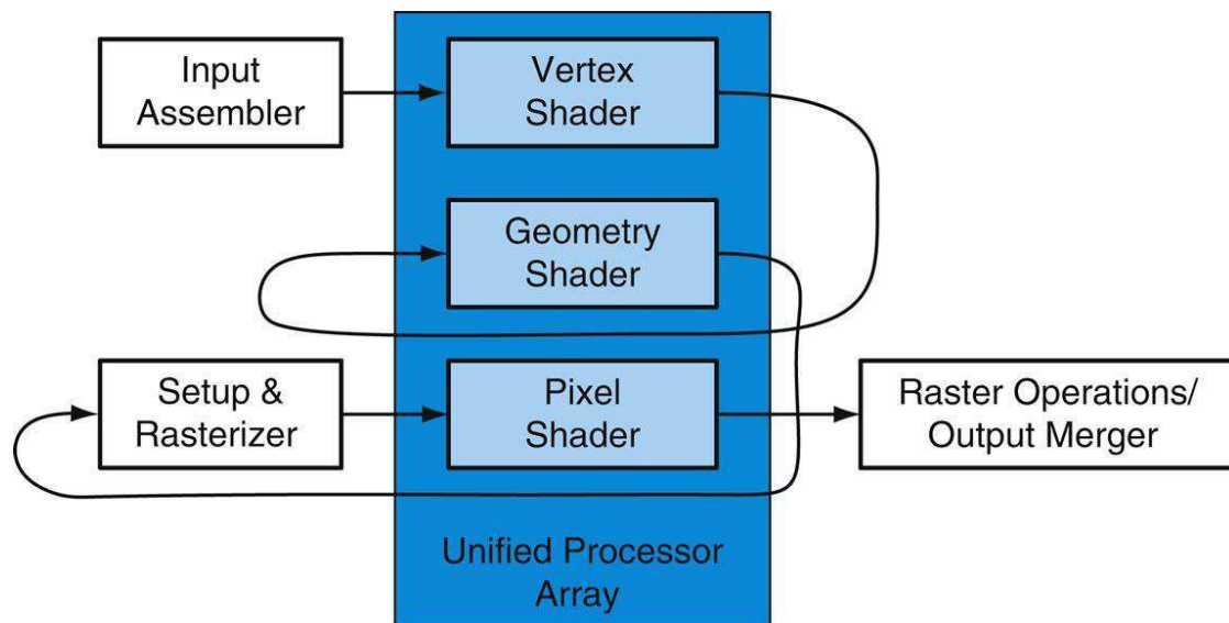
FIGURE B.2.4 Logical pipeline mapped to physical processors.
