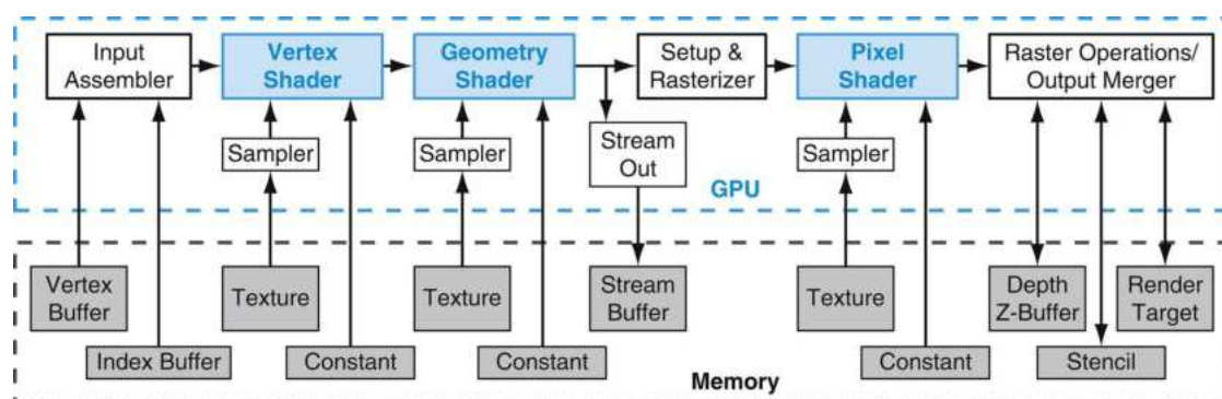
FIGURE B.3.1 Direct3D 10 graphics pipeline.
