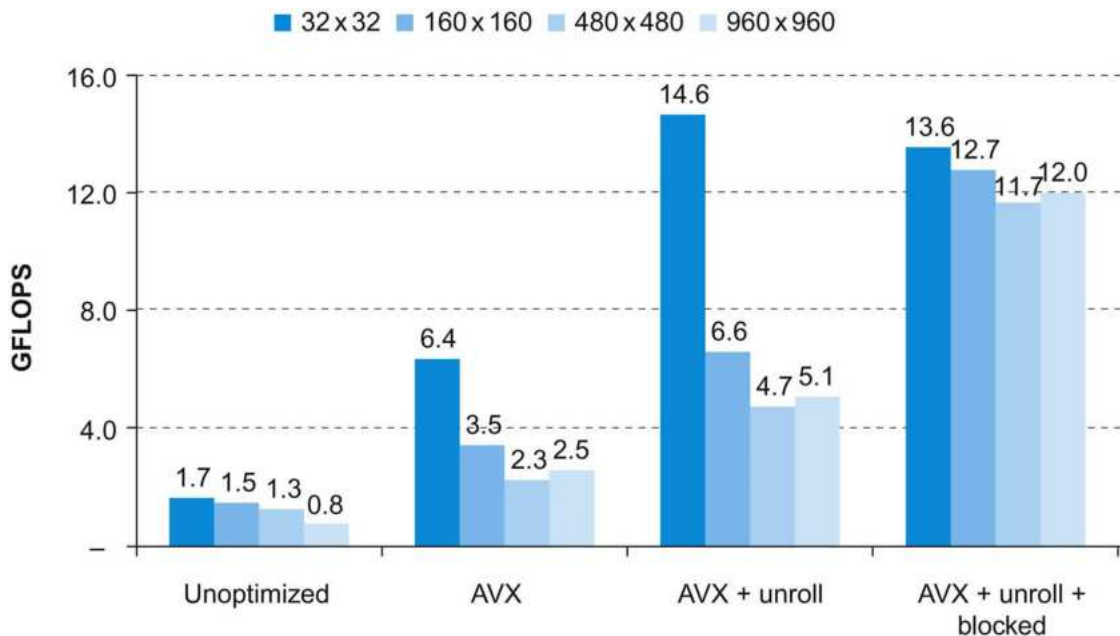
FIGURE 5.49 Performance of four versions of DGEMM from matrix dimensions 32 ×32 to 960 ×960.
