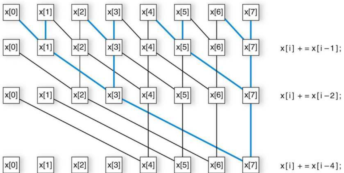
FIGURE B.8.8 Tree-based parallel scan data references.
