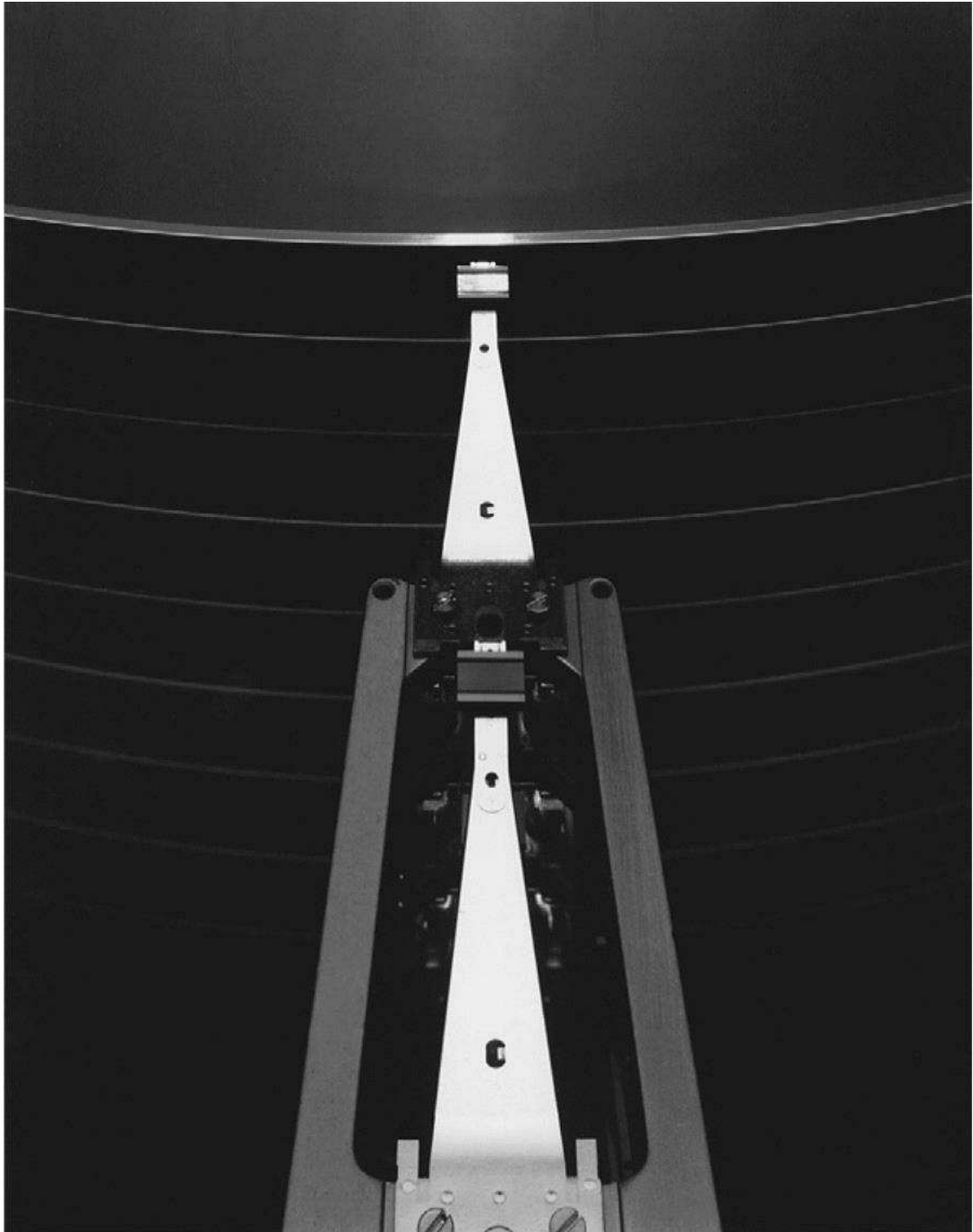
FIGURE 5.6 A disk showing 10 disk platters and the read/write heads.
