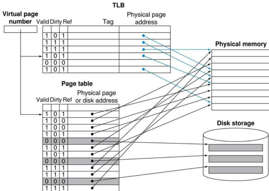
FIGURE 5.30 The TLB acts as a cache of the page table for the entries that map to physical pages only.
