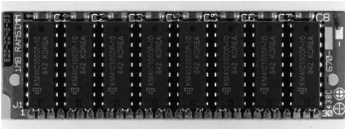
FIGURE E5.17.4 A 1 MB SIMM, built in 1986, using 1 Mbit chips.
