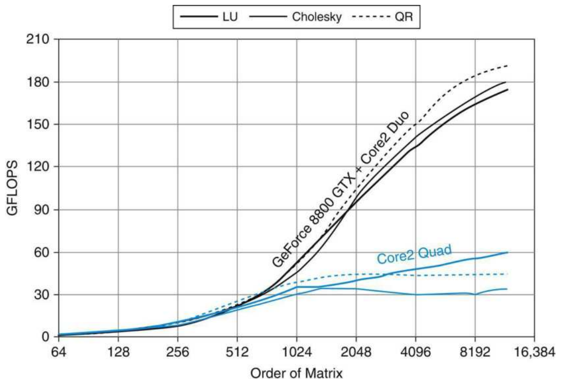
FIGURE B.7.4 Dense matrix factorization performance rates.
