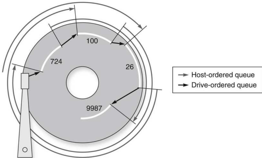
FIGURE 5.50 Example showing OS versus disk schedule accesses, labeled host-ordered versus drive-ordered.
