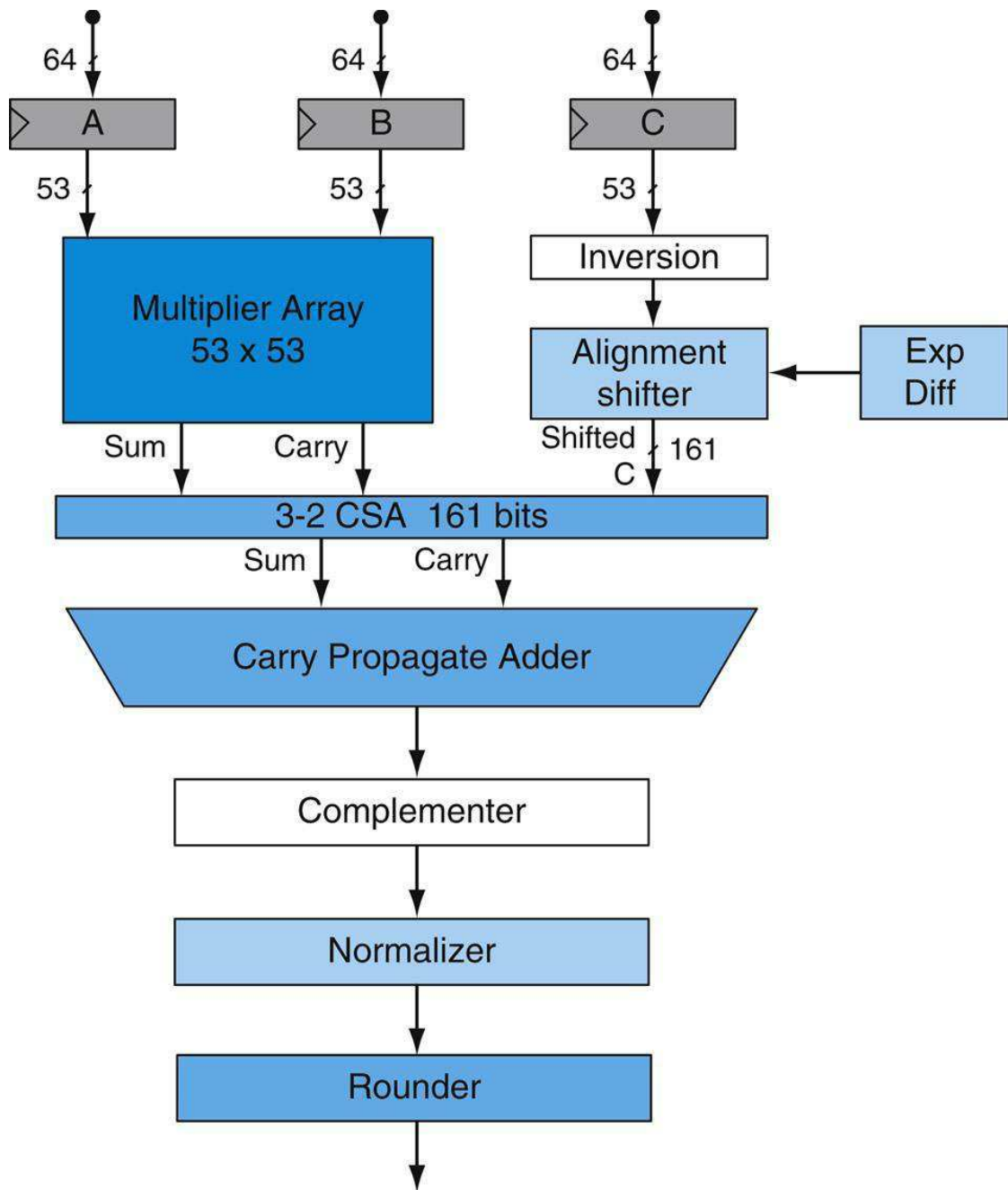
FIGURE B.6.2 Double-precision fused-multiply-add (FMA) unit.
