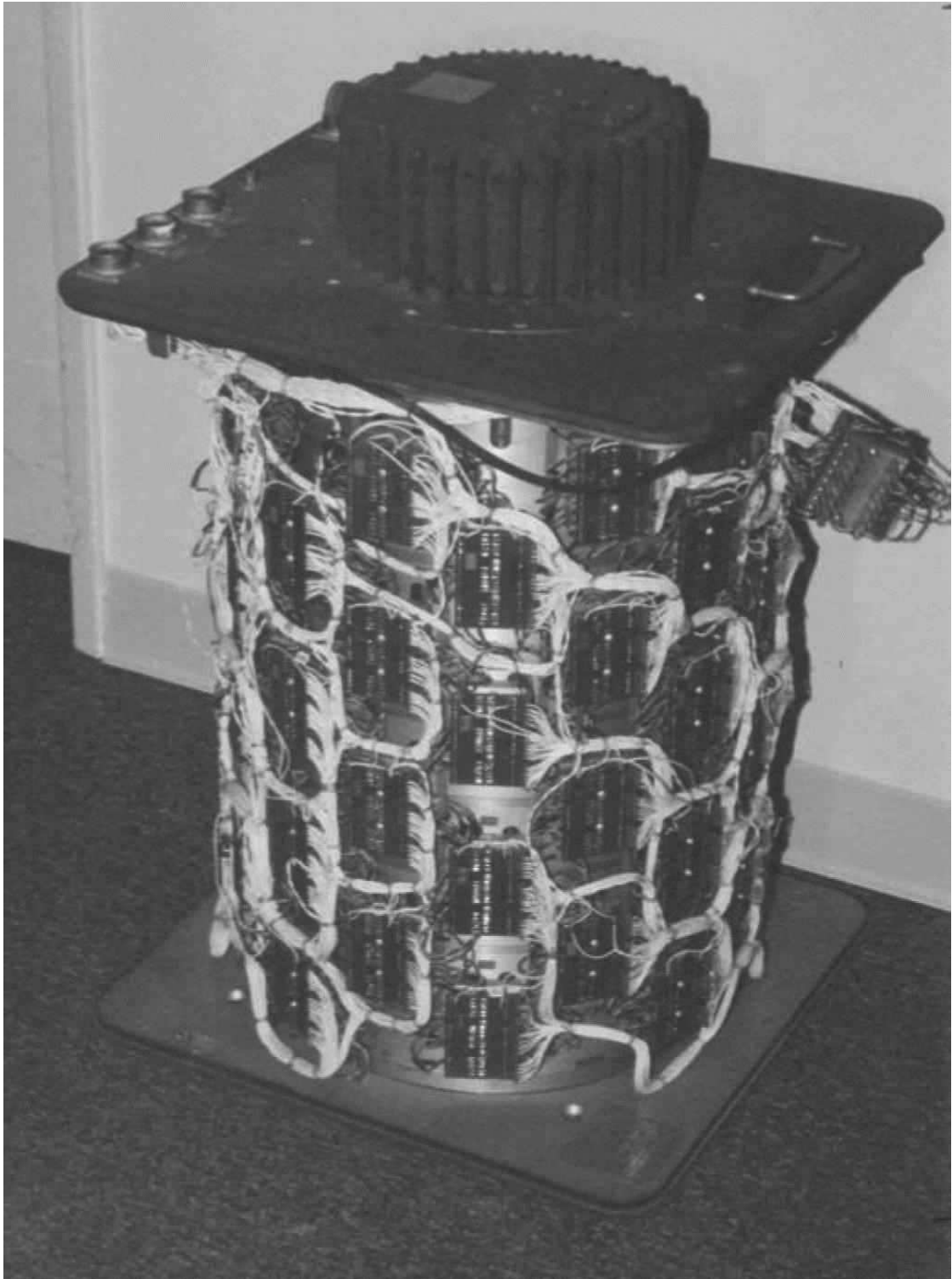
FIGURE E5.17.5 A magnetic drum made by Digital Development Corporation in the 1960s and used on a CDC machine.
