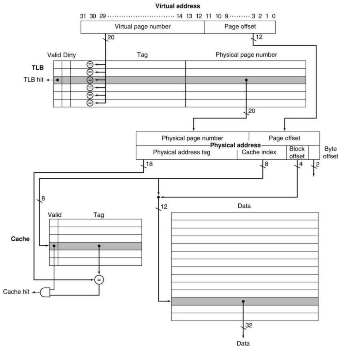
FIGURE 5.31 The TLB and cache implement the process of going from a virtual address to a data item in the Intrinsic FastMATH.
