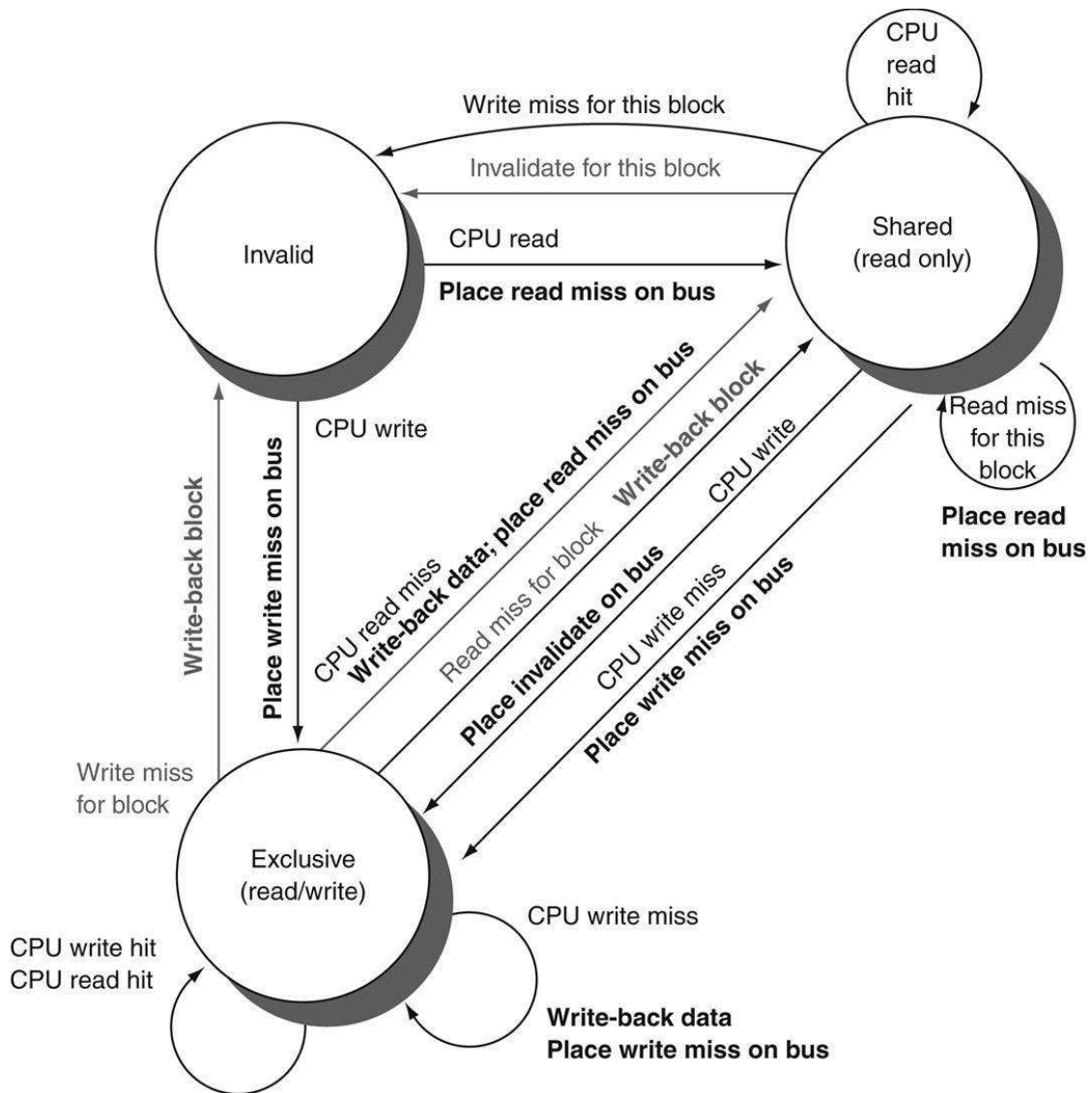
FIGURE E5.12.11 Cache coherence state diagram with the state transitions induced by the local processor shown in black and by the bus activities shown in gray.
