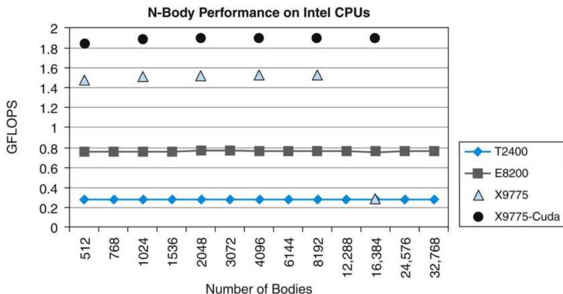
FIGURE B.8.16 Performance measurements on the N-body code on a CPU.
