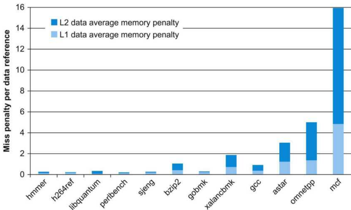
FIGURE 5.45 The average memory access penalty
