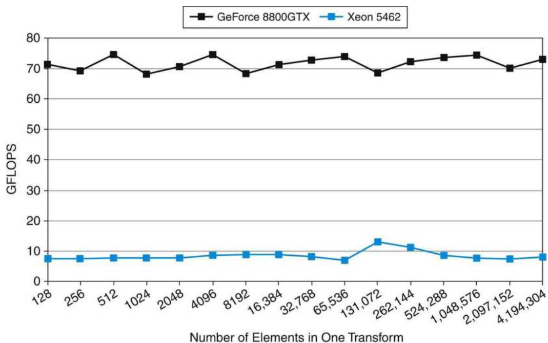
FIGURE B.7.5 Fast Fourier transform throughput performance.
