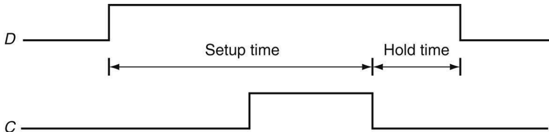
FIGURE A.8.6 Setup and hold time requirements for a D flip-flop with a falling-edge trigger.
