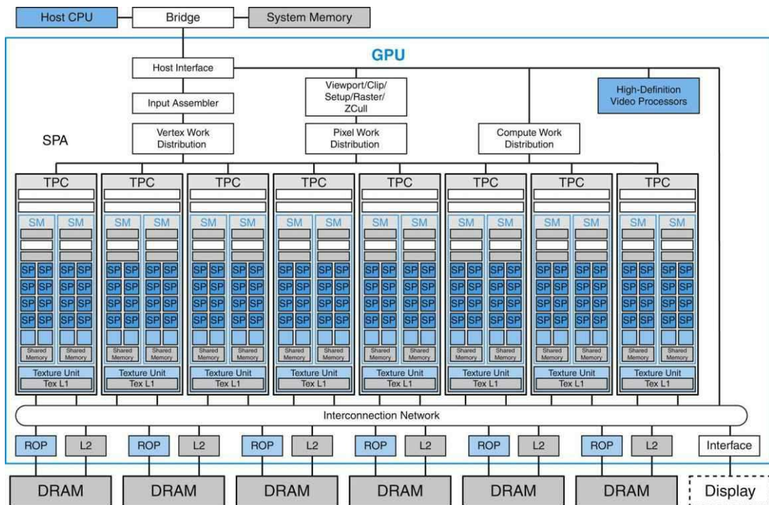
FIGURE B.7.1 NVIDIA Tesla unified graphics and computing GPU architecture.
