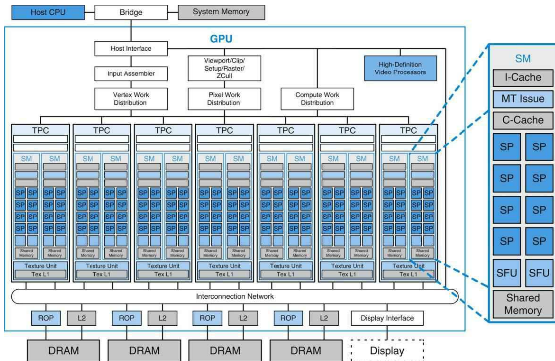
FIGURE B.2.5 Basic unified GPU architecture.
