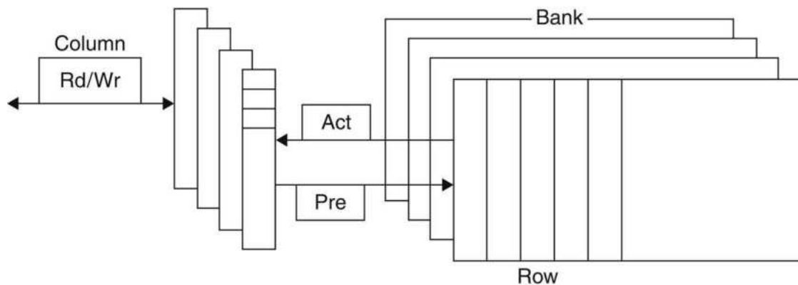
FIGURE 5.4 Internal organization of a DRAM.
