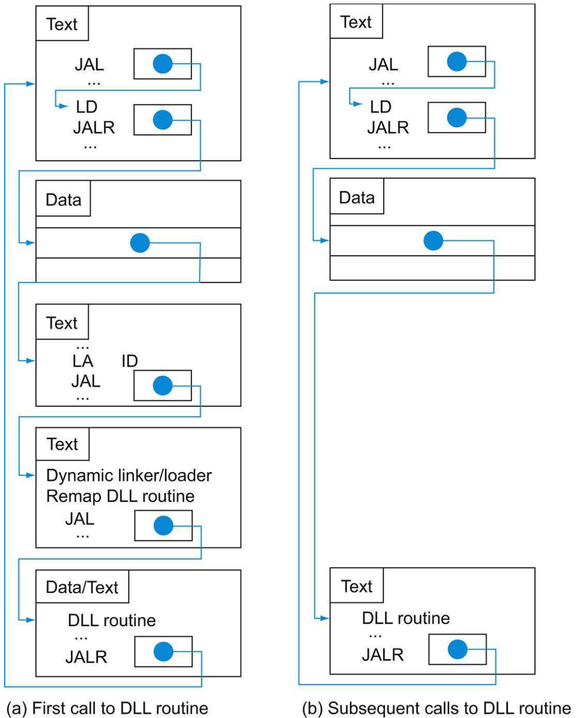
FIGURE 2.21 Dynamically linked library via lazy procedure linkage.
