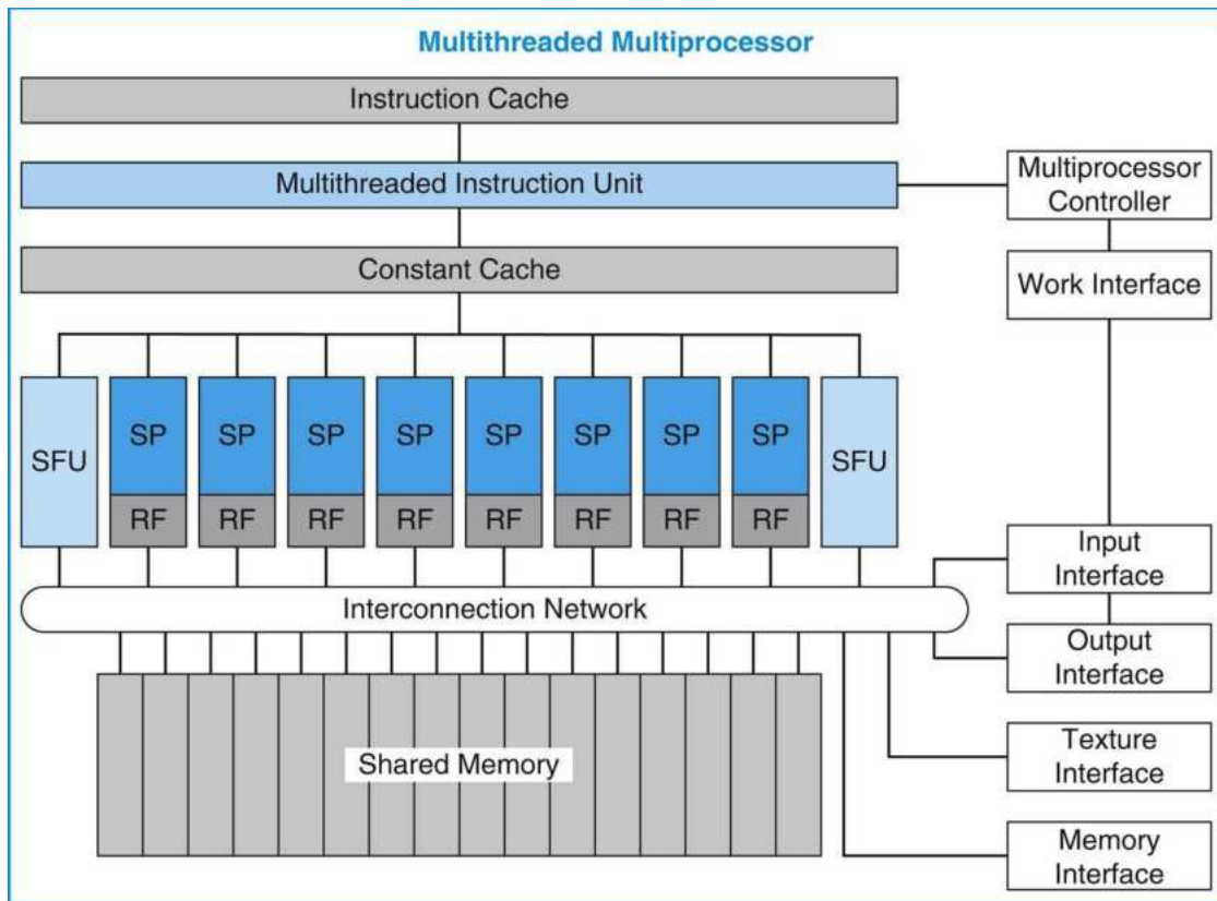
FIGURE B.4.1 Multithreaded multiprocessor with eight scalar processor (SP) cores.
