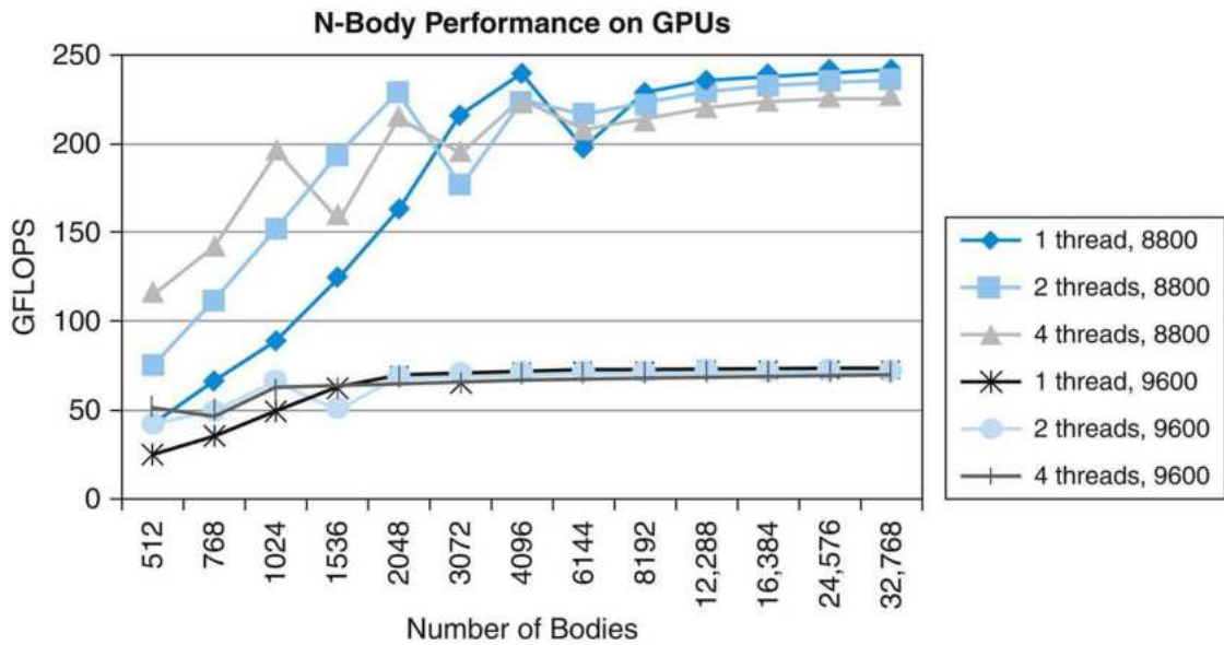
FIGURE B.8.15 Performance measurements of the N-body application on a GeForce 8800 GTX and a GeForce 9600.
